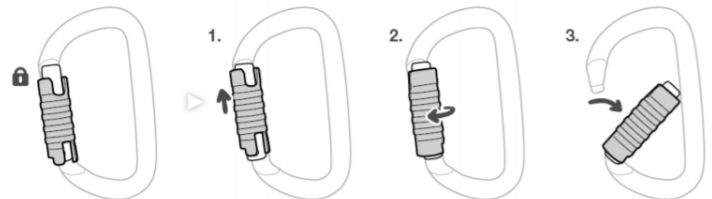
TRIACT-LOCK (TL)
